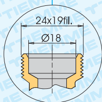
Art. 1716 Per tubo Pe-x For Pe-x pipe
