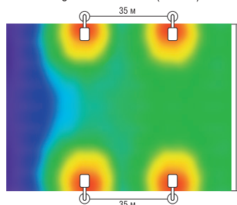
Navigator NSF-P-LED (200 Вт)
