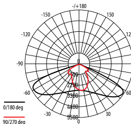
PSL-C-02-100W 5000K 10000Лм
