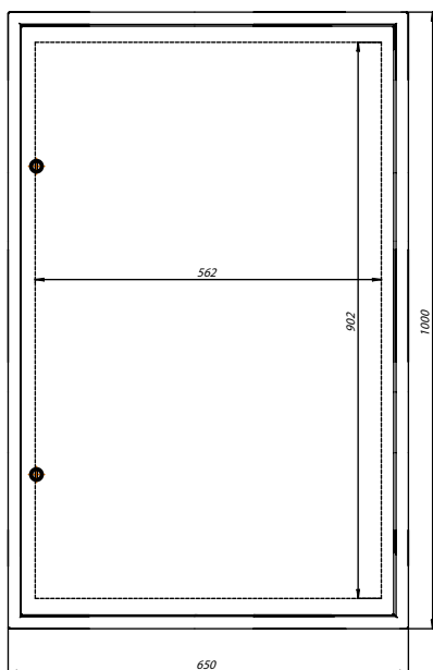
ЩМП-100x65x30
