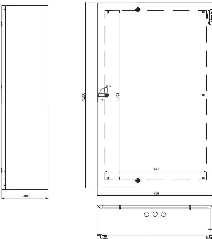
ЩМПГ-100x65x22
