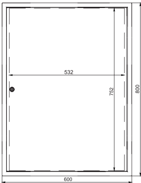
ЩМП-80x60x25
