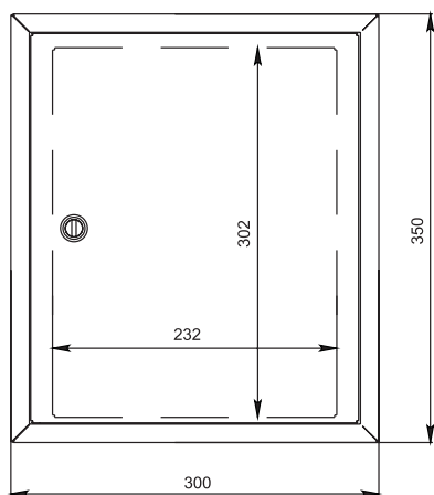
ЩМП-35x30x15
