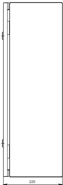
ЩМПГ-65x50x22
