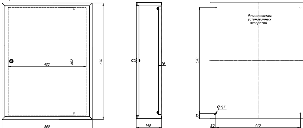
ЩМП-65x50x22
