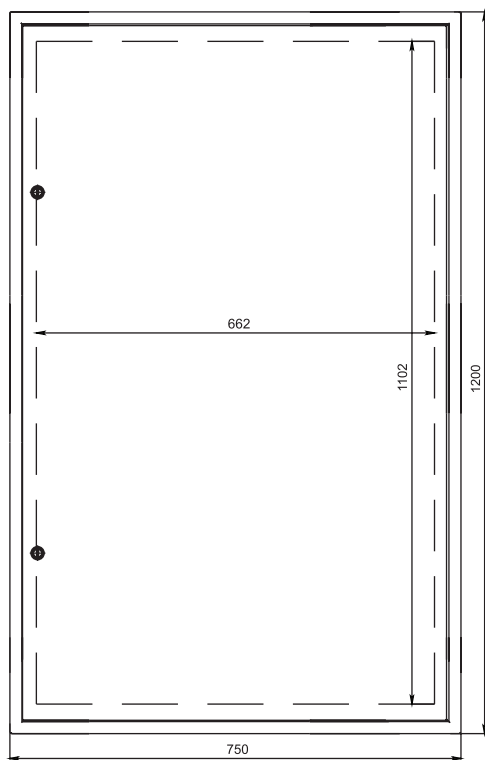
ЩМП-120x75x30
