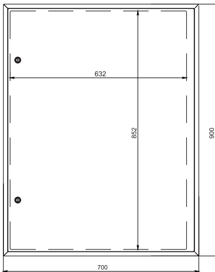
ЩМП-90x70x26
