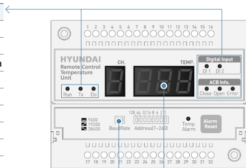
Communication setting Temperature signal
