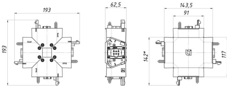
X-connector DOMINO
