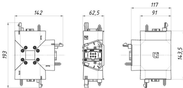
T-connector DOMINO
