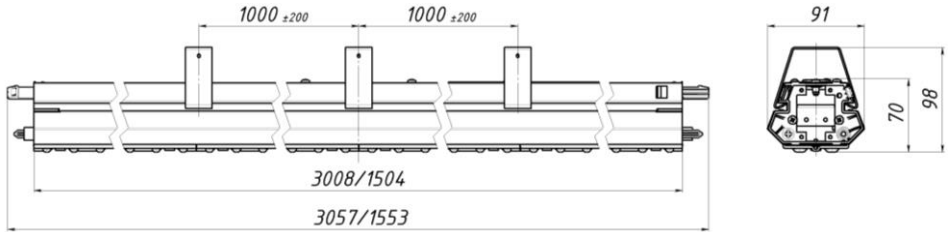
DOMINO LED 2x40 (2x80) D90 4000K / DOMINO LED 40 (80) D90 (HFR) 4000K
